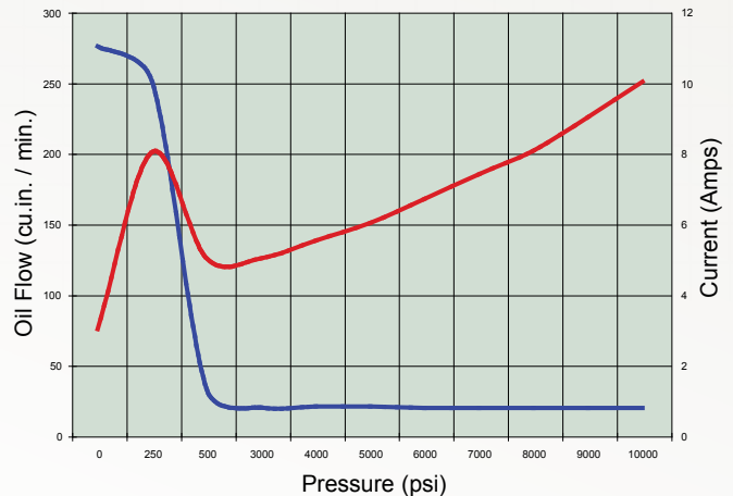
Performance Chart
