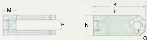
Pull Cylinder Dimensions
