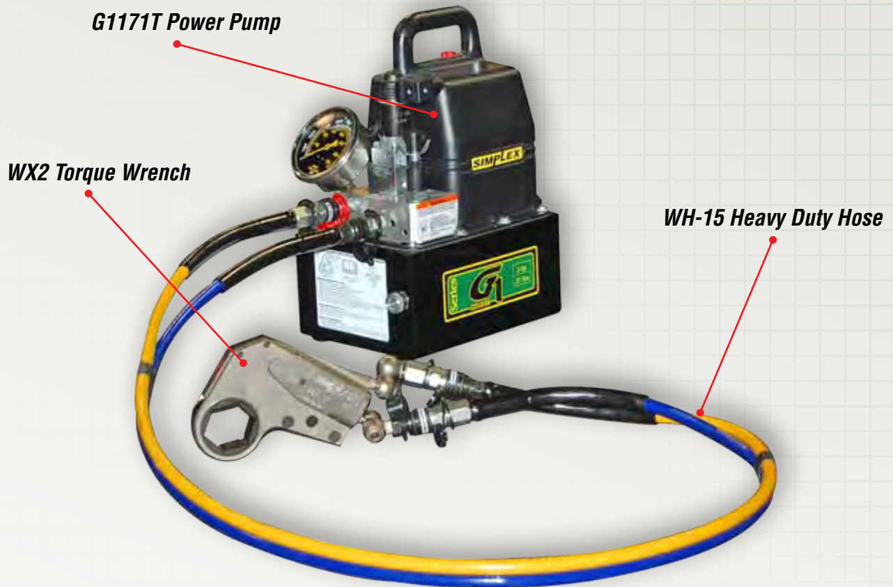
Standard Bolting Model Shown
