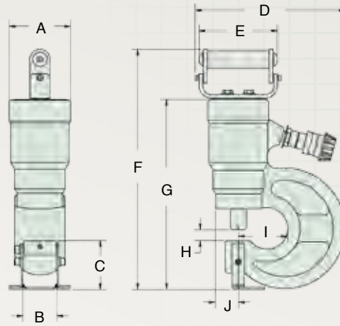
Punch Dimensions
