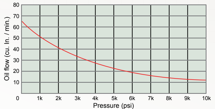
Performance Chart
