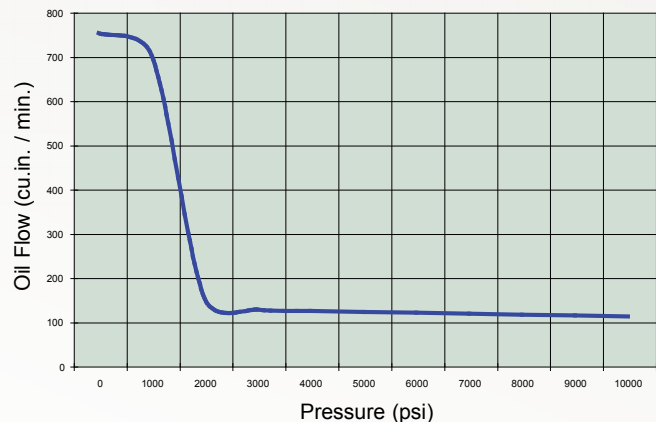
Performance Chart
